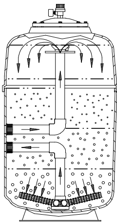
Abb. B-2: Filtration GENO-mat® F 600
